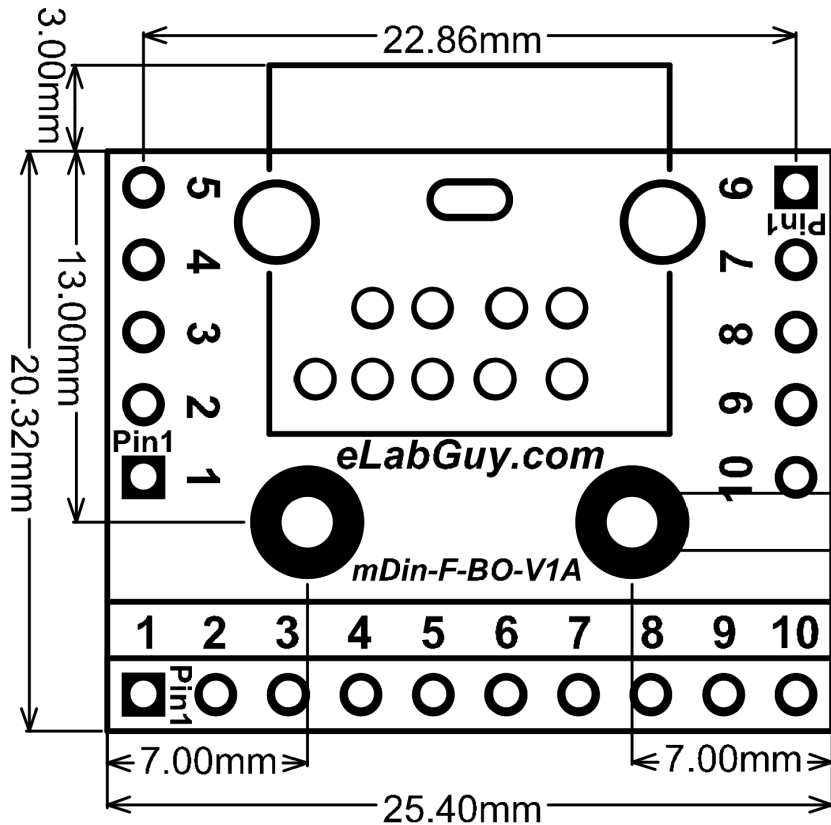
mDin-F-BO-V1A PCB outline Drawing
